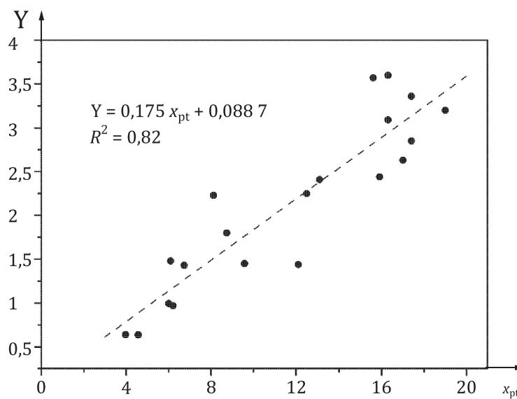
Figure E.8 — Relative standard deviation of participant results (%) vs assigned reference value ( \mu\text{g/l} )
